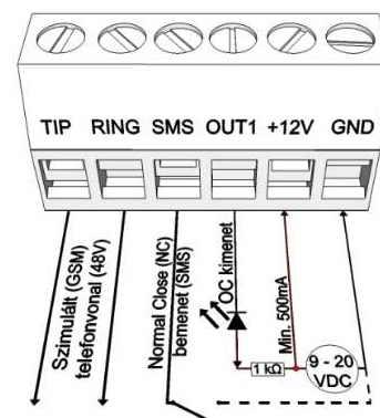
Wiring diagram
